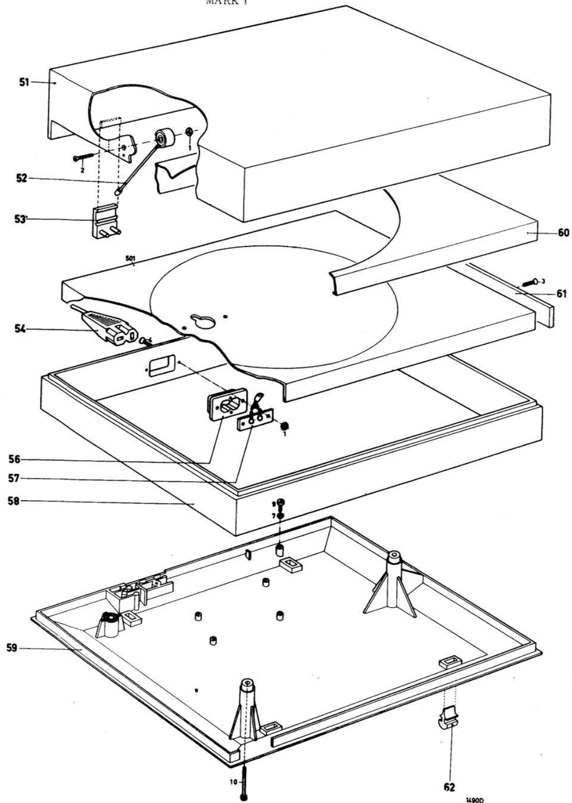
List of mechanical parts (cabinet) Mark I
