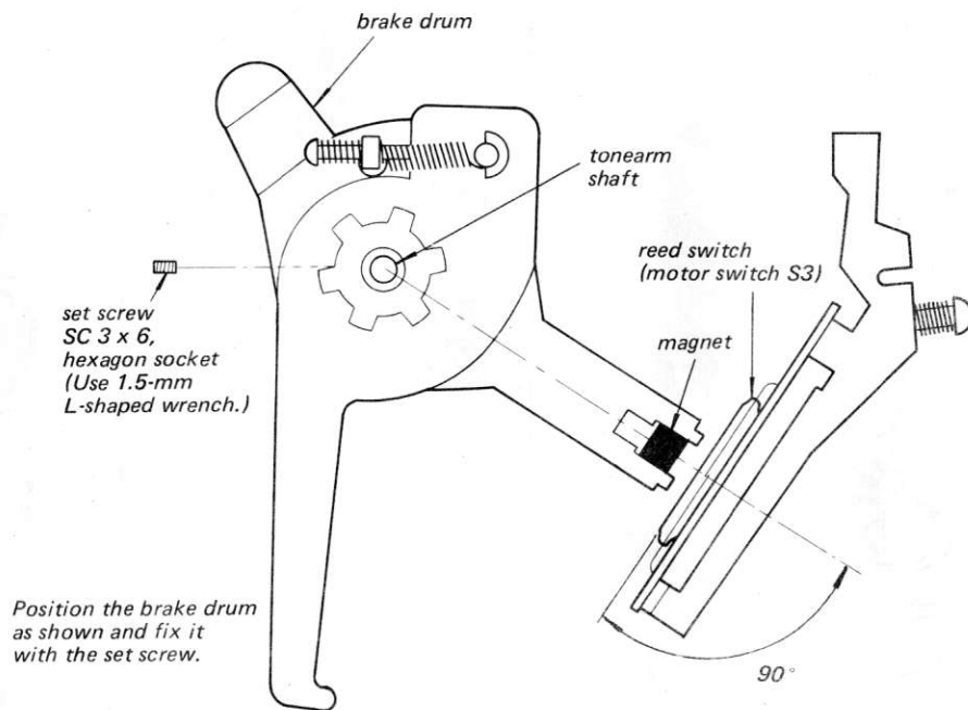
Reed Switch Mounting
