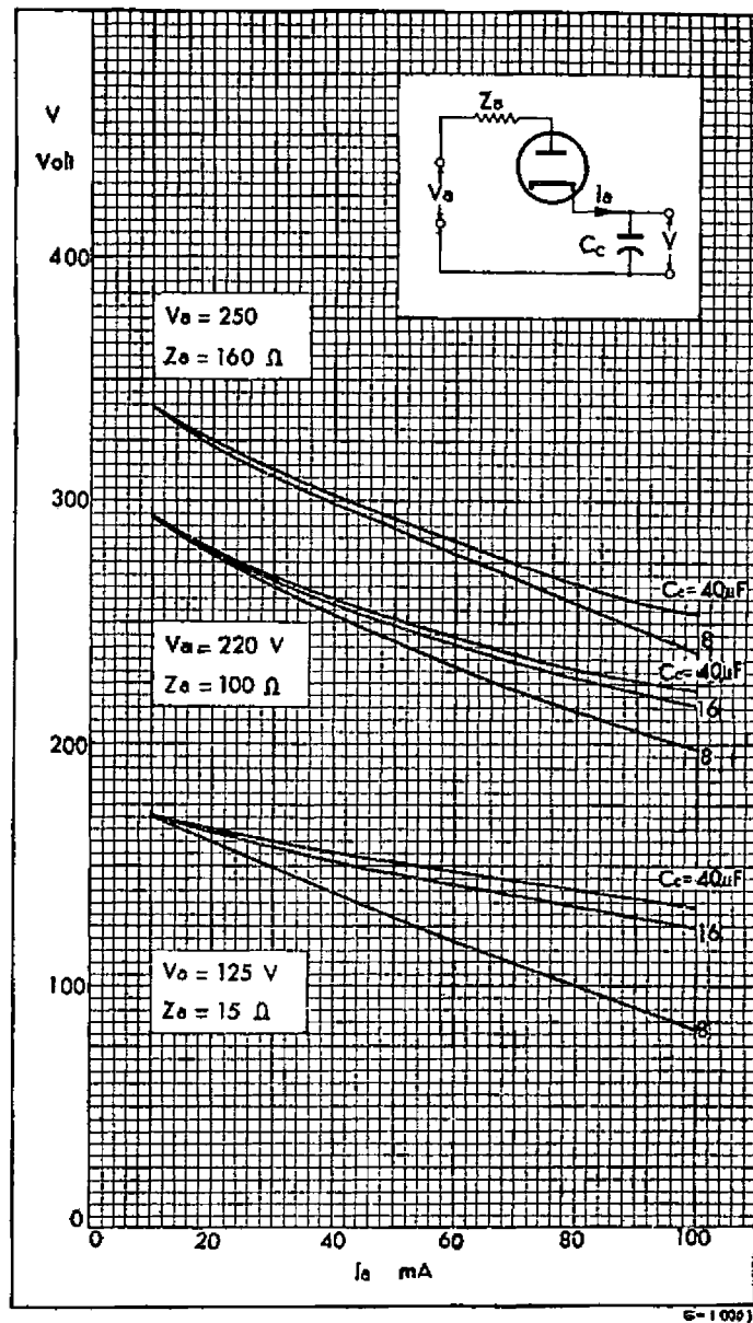
Fig. 1 — Operation Characteristics
