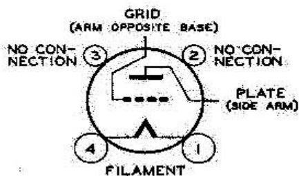
TUBE SYMBOL & TOP VIEW OF SOCKET CONNECTIONS
