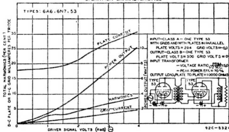
OPERATION CHARACTERISTICS
