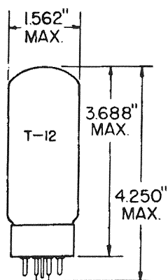
GLASS BULB SHORT MEDIUM SHELL 6 PIN OCTAL B6-248 LOW LOSS MATERIAL OUTLINE DRAWING JEDEC 17-15
