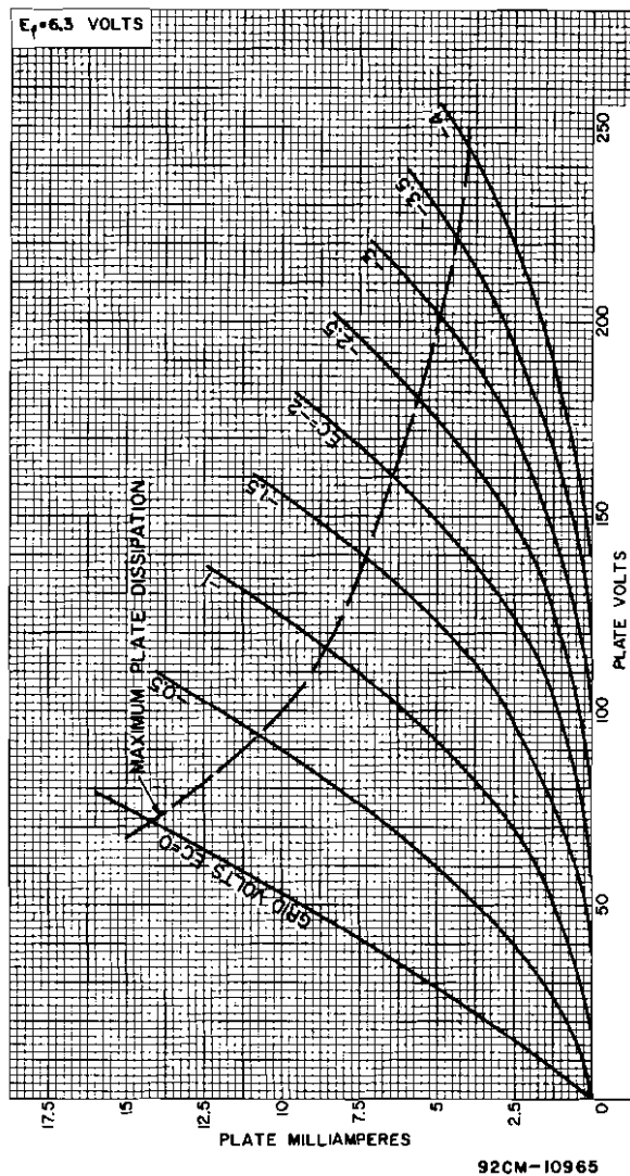
Fig. 1 - Average Plate Characteristics for Type 7895.
