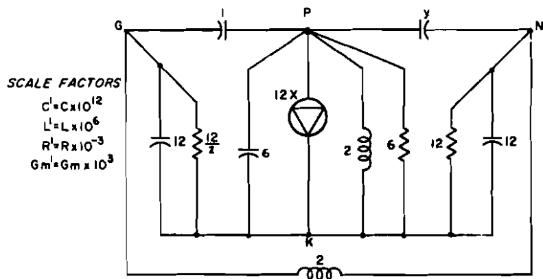
Fig. 3 - Tapped-capacitor neutralization circuit having typical Nuviator impedance values.
