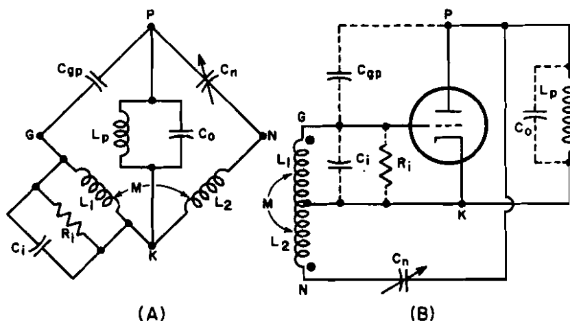
Fig. 1 - Basic tapped-coil arrangement for triode neutralization (Rice system of neutralization).
