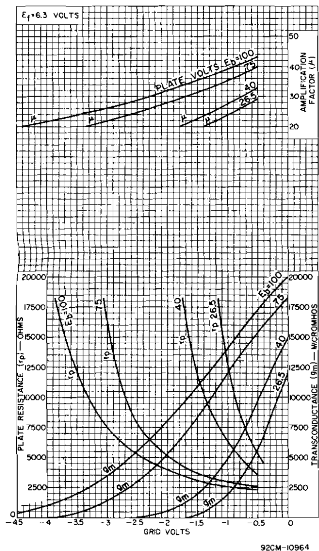
Fig.5 - Average Characteristics for Type 7586.
