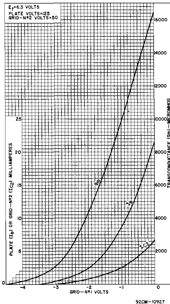
Fig.2 - Average Characteristics for Type 7587.
