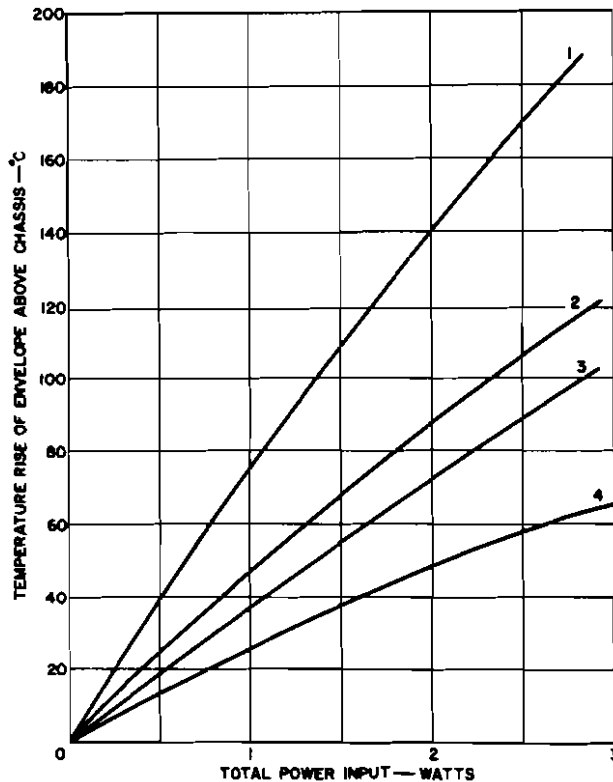
Fig.6 - Temperature curves for developmental long-lead nuvistor triodes: (1) in free air, no socket, not mounted; (2) in free air, no socket, August Heat Dissipator; (3) mounted in IERC clamp, attached to printed board, no socket; (4) mounted in IERC clamp, attached to heat sink, no socket.
