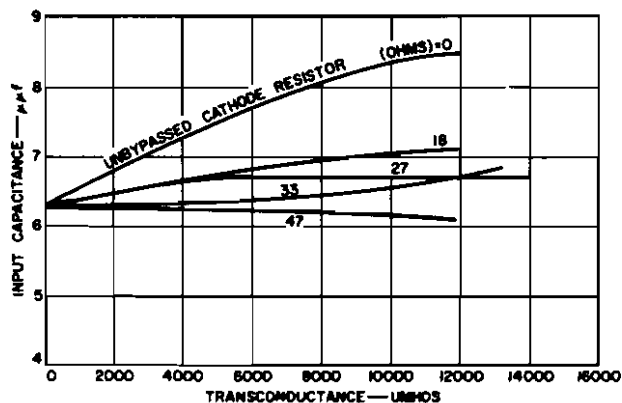
Fig. 4 - Short-circuit input-loading data for Nuvistor triode.
