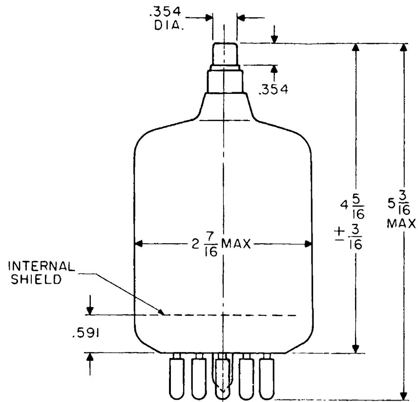
GIANT 5 PIN BASE
