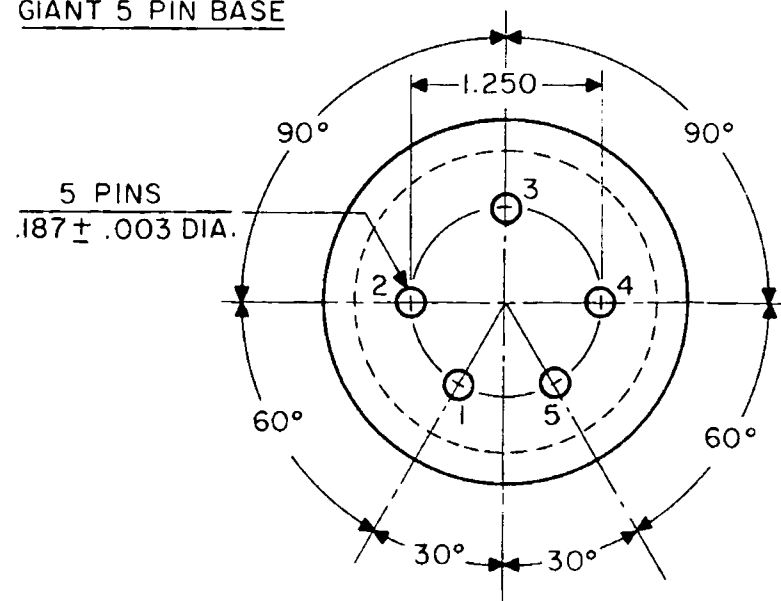
GIANT 5 PIN BASE
