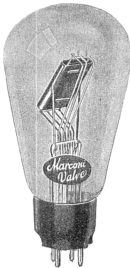
Marconi P 625 & P 625a Super Power Output Valve
