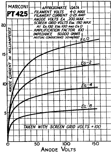
Screen Volts 100
