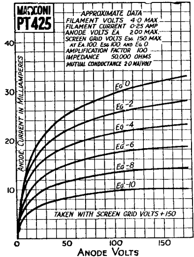
Screen Volts 150
