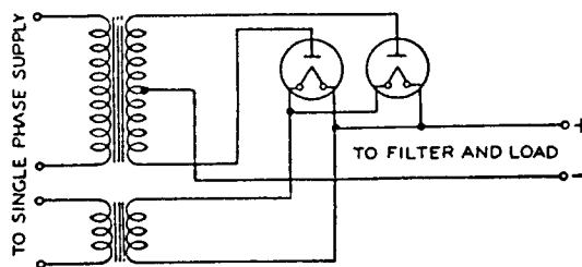
SINGLE PHASE, DOUBLE HALF-WAVE CIRCUIT B
