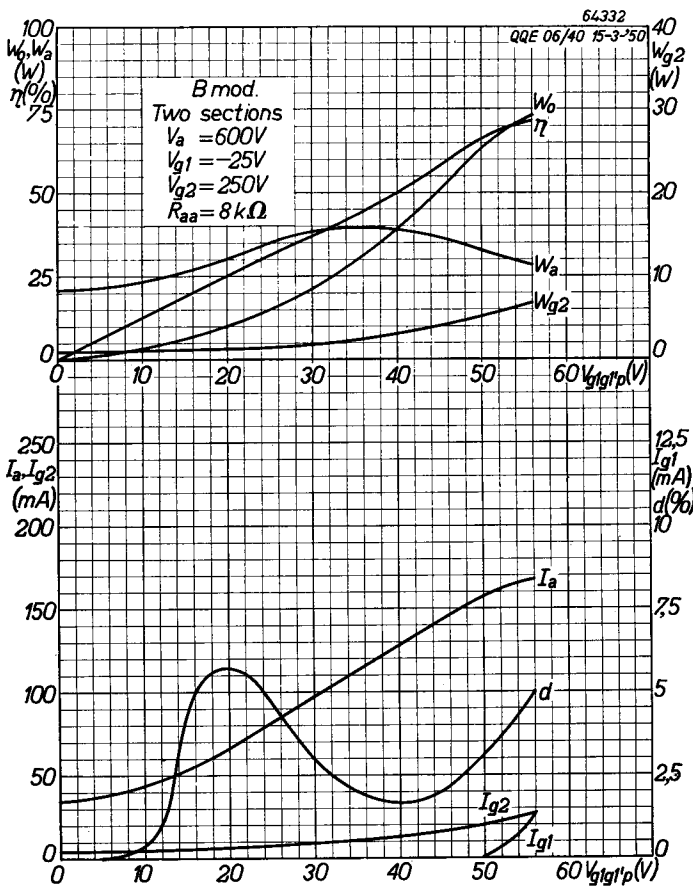
Fig. 13. Curves showing the performance as A.F. amplifier and modulator in push-pull class B. Anode current I_a , screen-grid current I_{g2} , control-grid current I_{g1} , output power W_o , anode dissipation W_a , screen-grid dissipation W_{g2} , distortion d_{tot} and efficiency \eta are plotted against the peak-to-peak value of the input voltage.
