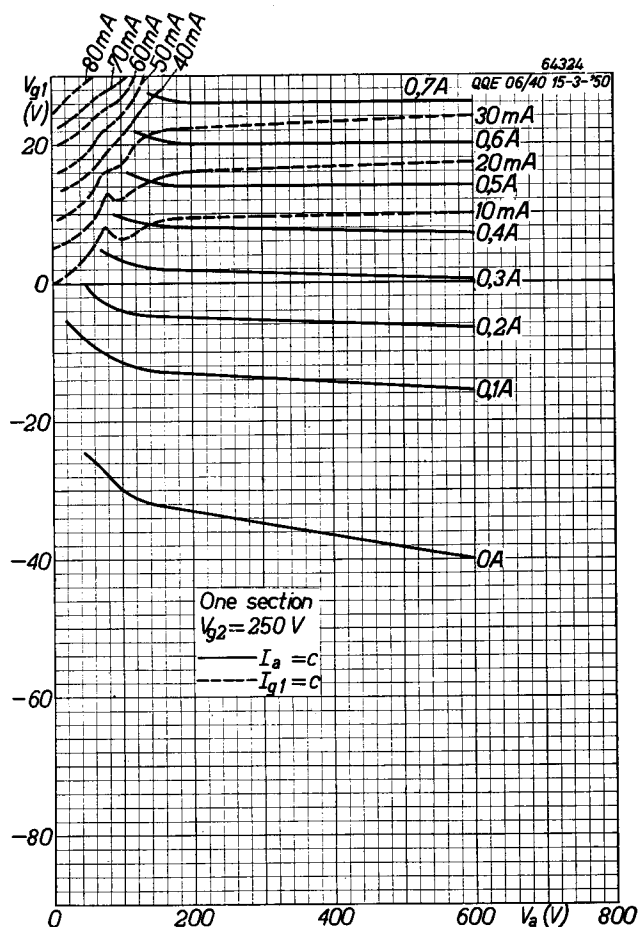
Fig. 5. Control-grid voltage V_{g1} as a function of the anode voltage V_a at constant anode current I_a and constant control-grid current I_{g1} for a screen-grid voltage V_{g2} of 250 V.
