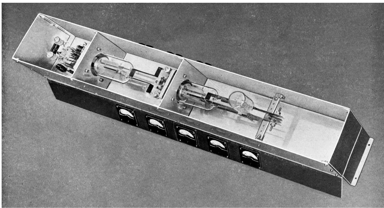
Fig. 16. Photograph of the 30 W power amplifier with QQE 06/40 at 430 Mc/s. Left compartment: oscillator stage with QQC 04/15. Middle compartment: tripler stage with QQE 06/40. Right compartment: final amplifier with QQE 06/40.
