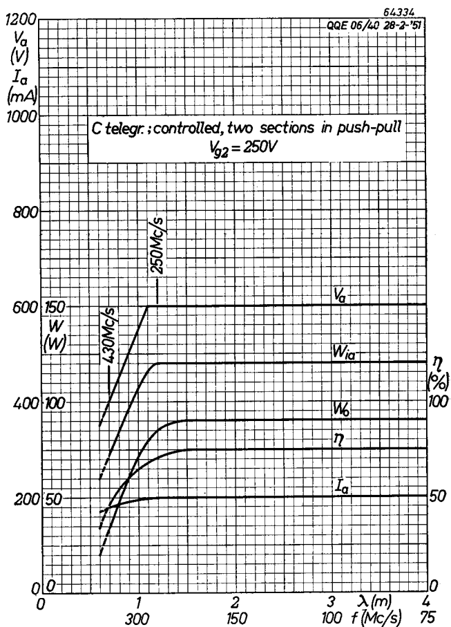
Fig. 15. Anode supply power W_{ia} , output W_o , permissible anode voltage V_a , efficiency \eta and anode current I_a as functions of frequency and wavelength for the two sections in push-pull under C telegraphy operating conditions.
