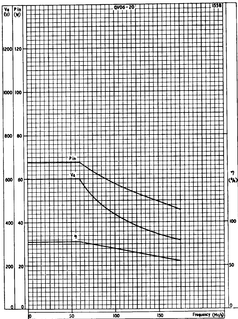
FREQUENCY CHARACTERISTICS
