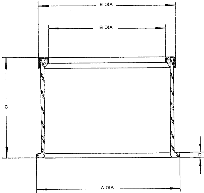
GC11 Outline
