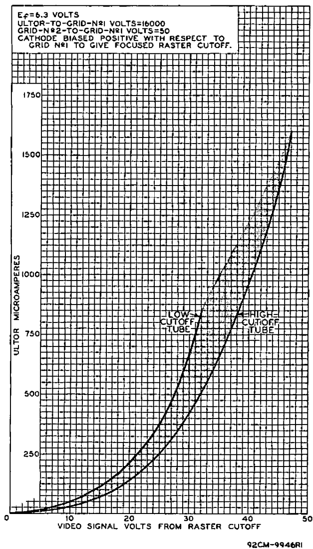
Fig. 3 - Cathode-Drive Characteristics of Type 23NP 4 .
