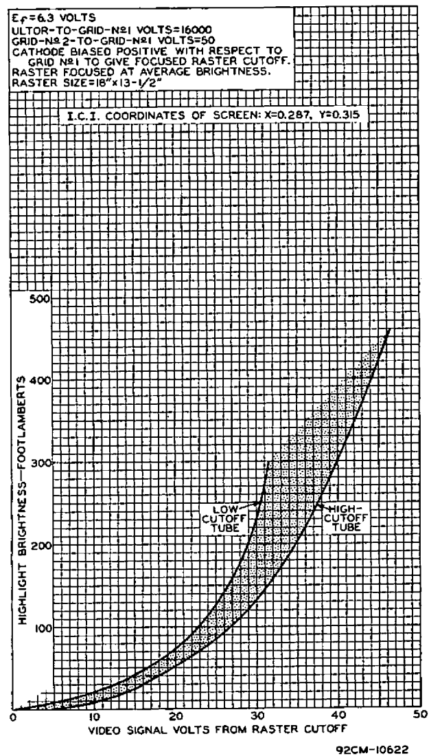
Fig. 4 - Cathode Drive Characteristics of Type 23NP 4 .
