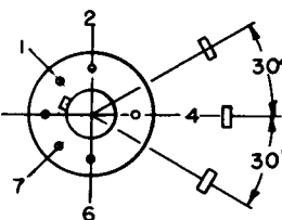
BOTTOM VIEW OF BASE (NOTE-2)
