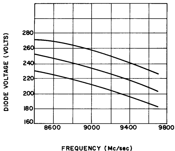
TYPICAL TUNER DIODE VOLTAGE VS FREQUENCY
