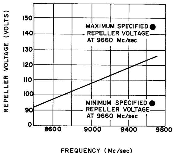
TYPICAL VARIATION OF REPELLER VOLTAGE VS FREQUENCY
