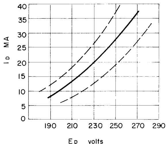
STATIC DIODE CHARACTERISTICS
