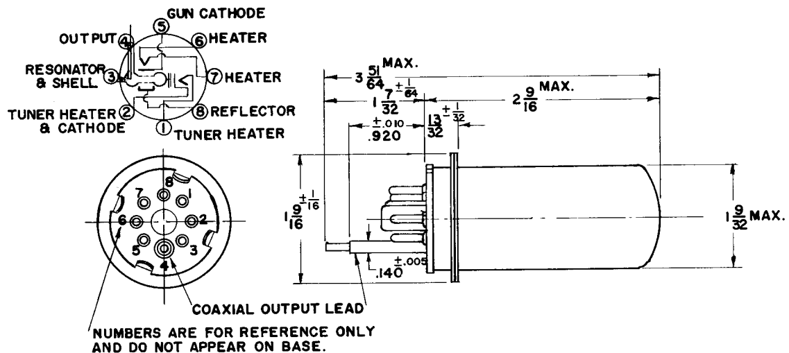
OUTLINE DRAWING
