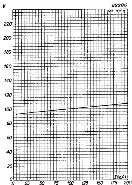
Fig. 5 Voltage-current characteristic of the 13201.
