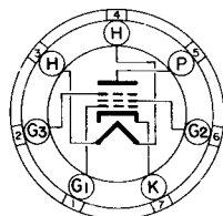
BOTTOM VIEW MINIATURE BUTTON 7 PIN BASE TCC
