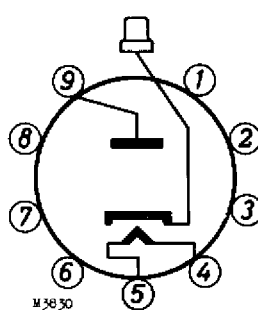
BOTTOM VIEW OF BASE
