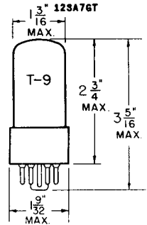
GLASS BULB
