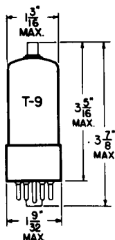
GLASS BULB
