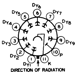
TERMINAL DIAGRAM (Bottom View)
