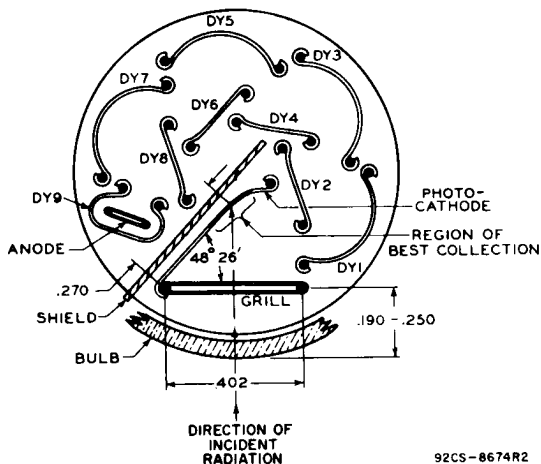
DETAIL A (Top View)
