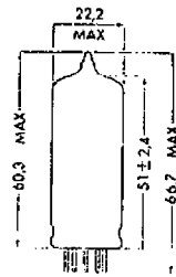
Dimensions in millimeters
