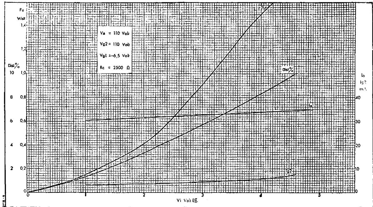
Fig. 3 — Average Characteristics
