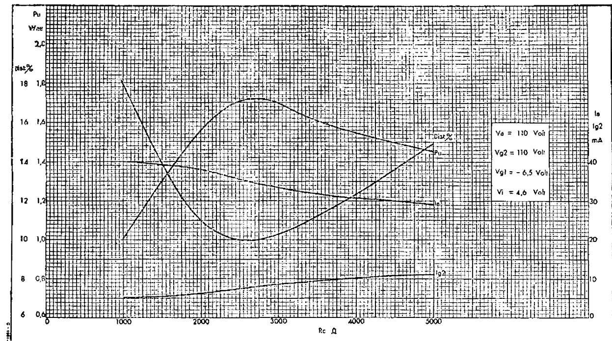
Fig. 4 — Average Characteristics
