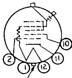
BOTTOM VIEW OF BASE 12 AT
