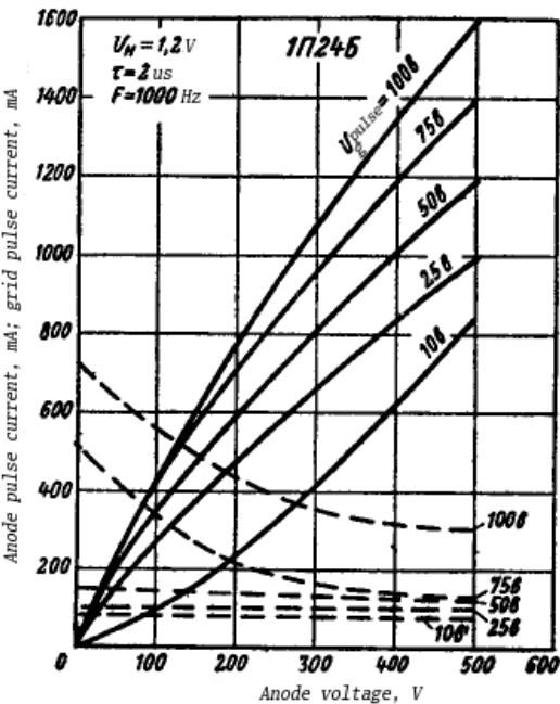
Pulsed characteristics in triode connection
