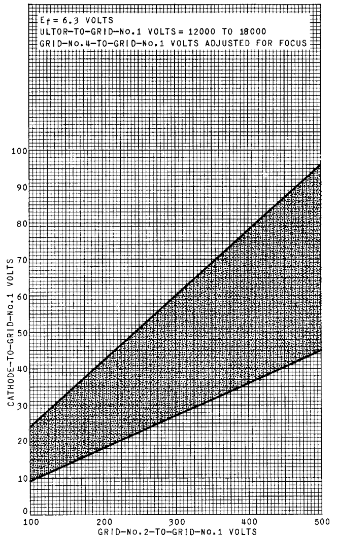
Fig. 2 - Raster Cutoff Range for Type 21CEP4 in Cathode-Drive Service.
