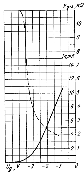
I_a R_{g1k} = f(U_{gT}) (второго триода) (for the second triode) — — — I_a U_h = 6,3 \text{ V} - - - - R_{g1k} U_a = 90 \text{ V} f = 210 \text{ MHz}
