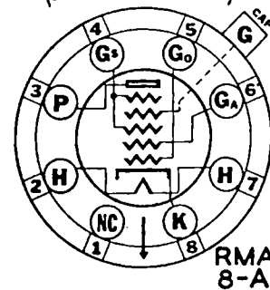
TUBE AND BASE DIAGRAM (BOTTOM VIEW)
