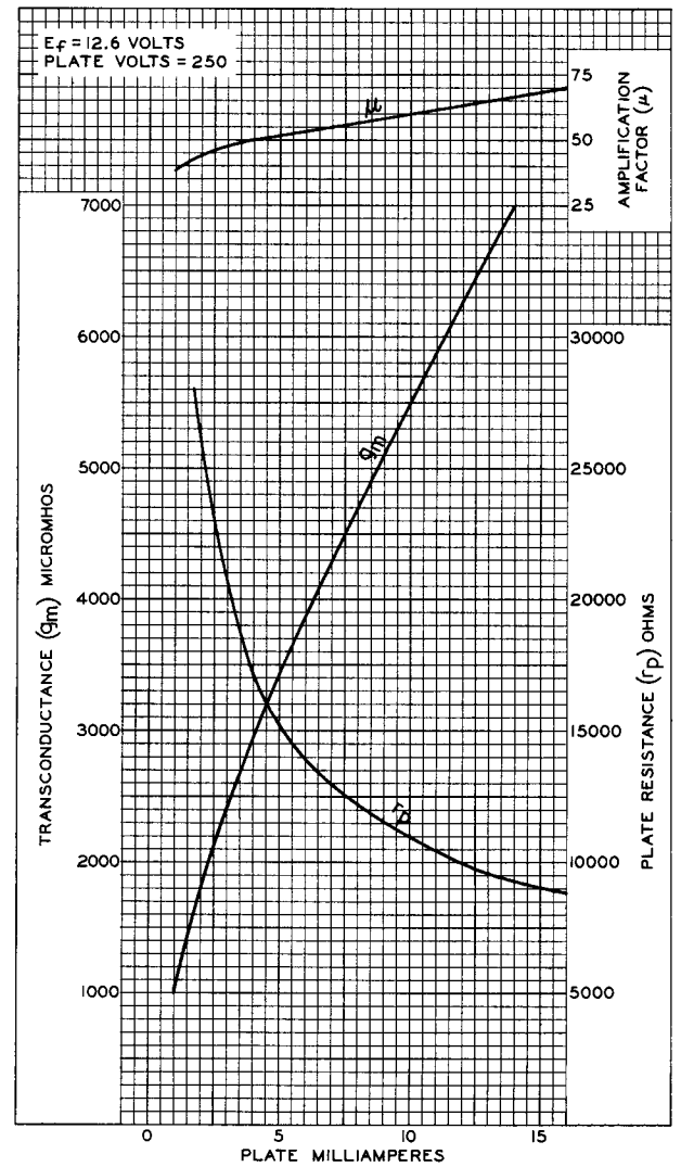
Fig. 2 - Average Characteristics of Type 12DT8.
