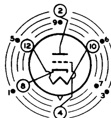
INDEX-LARGE LUG ●=SHORT PIN
