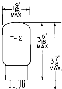
GLASS BULB
