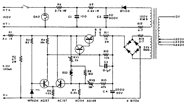
FIG. 2. POWER SUPPLY
