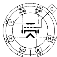
G-7V BOTTOM VIEW 6R7G, 6R7GT
