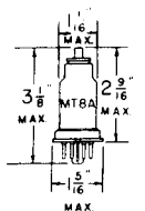
METAL SHELL SMALL WAFER 7 PIN OCTAL BASE 6R7
