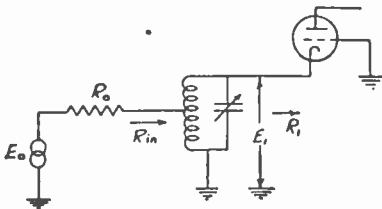
Fig. 6—Antenna input circuit for grounded-grid amplifier.
