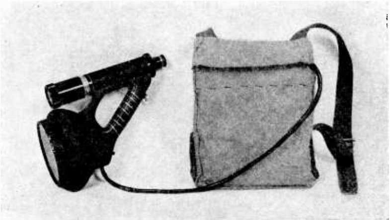
Fig. 9—Laboratory prototype Snooperscope.
