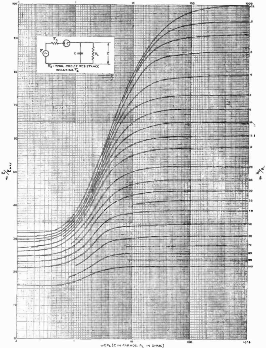
Fig. 3—Relation of applied alternating peak voltage to direct output voltage in half-wave, condenser-input circuits.
