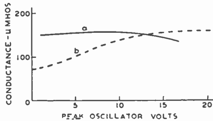
Fig. 17—Signal-grid (grid No. 1) conductance of typical mixer designed for outer-grid injection of oscillator. Frequency, 31.5 megacycles, signal-grid bias, E_{r1} = -3 volts. Curve a corresponds to fixed No. 3 grid bias, E_{r3} = -8 volts. Curve b corresponds to bias through a 50,000-ohm grid leak.
