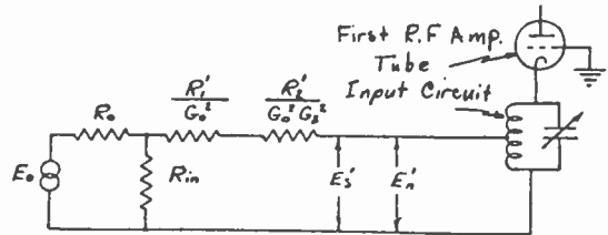
Fig. 10—Noise sources within a receiver.
