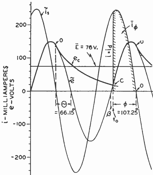
Fig. 27—Graphic solution of operation for a half-wave, condenser-input circuit without series resistance.
