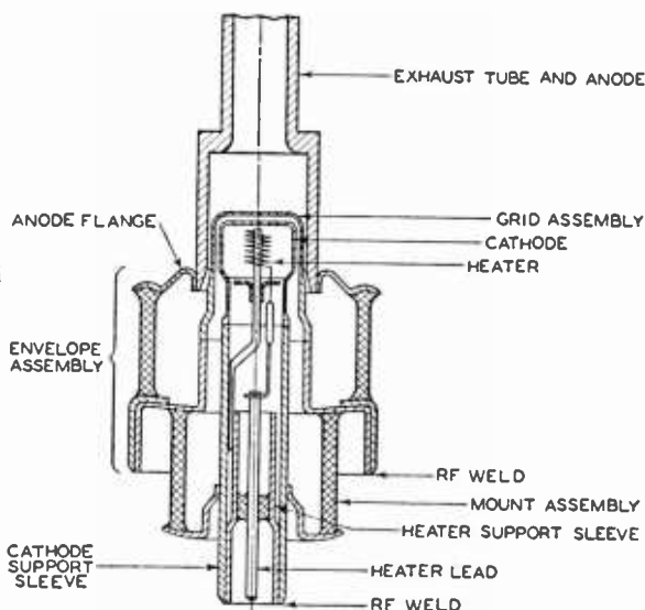
Fig. 1—Cross-sectional view of the 5588.
