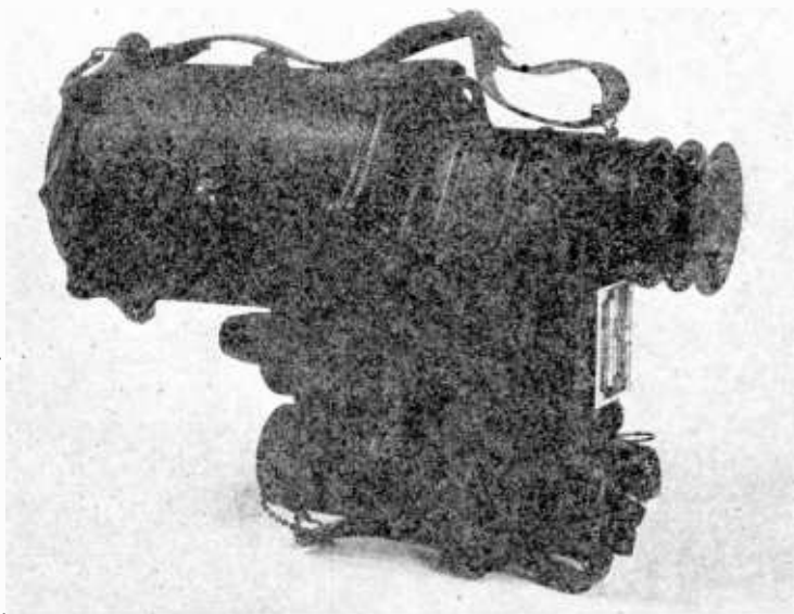
Fig. 1—Infrared telescope.
