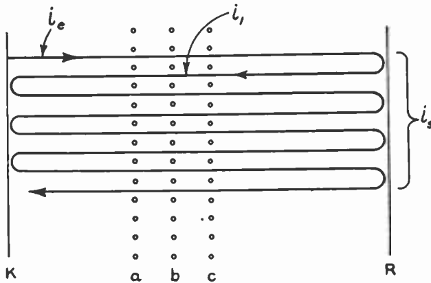
Fig. 2—Schematic electron paths in a triple-grid reflex oscillator, showing the effective current i_e and the built-up space current i_s , due to multiple transits, between cathode K and reflector R .
