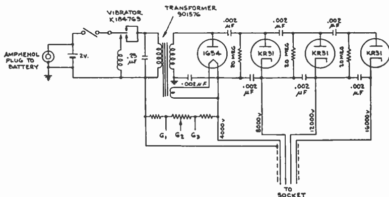
Fig. 22—Circuit of voltage quadrupler power supply (Type S-5).
