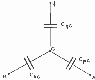
Fig. 6—Star network of the capacitances of the triode of Fig. 5.
