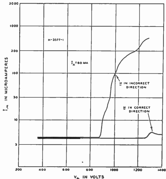
Fig. 5 — Noise in magnetron with grooved cathode. When the magnetic field is in the "correct" direction, the oxide-coated surfaces are sheltered from back-bombarding electrons.
