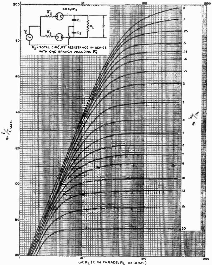
Fig. 5—Relation of applied alternating peak voltage to direct output voltage in condenser-input, voltage-doubling circuits.
