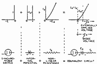
Fig. 1—Characteristics and equivalent circuit for high-vacuum diodes.
