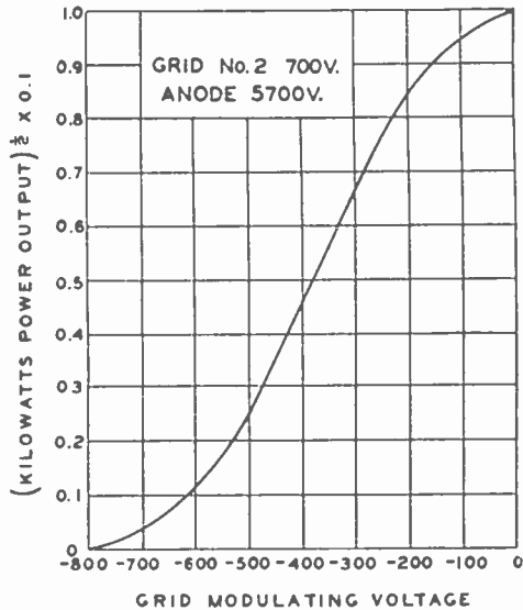
Fig. 11— Modulation characteristics.
