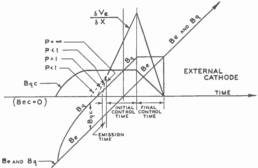
Fig. 4—Time variation of the magnetic field, magnetic flux and electric field. equilibrium orbit x_i , must be closer to the cathode than the anode;
