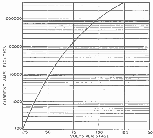
Fig. 2—Average amplification of type 931-A.
