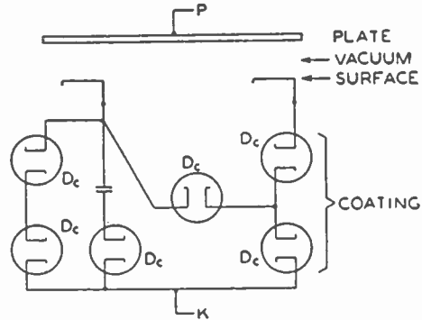
Fig. 18—Same as Fig. 17 with resistances replaced by special diodes.
