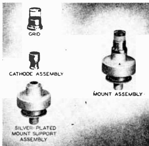
Fig. 5—Mount assembly and components.
