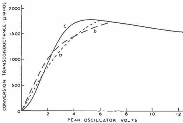
Fig. 5—Conversion transconductance of a typical variable- \mu radio-frequency pentode. Oscillator and signal voltages both applied to grid No. 1. a , fixed-bias operation; b , cathode resistor used to obtain bias; c , bias obtained by means of a high-resistance grid leak.
