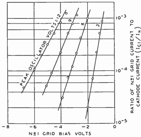
Fig. 15—Signal-grid (grid No. 1) current in a typical mixer with a 20-mega-cycle oscillator voltage applied to grid No. 3. E_{c3} = -10 volts. E_{c2} and c_1 = 100 volts, E_b = 250 volts.
