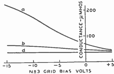
Fig. 19—Signal-grid (grid No. 1) conductance of the outer-grid-injection mixers shown in Fig. 18. Data taken at 31.5 megacycles with no oscillator voltage applied.
