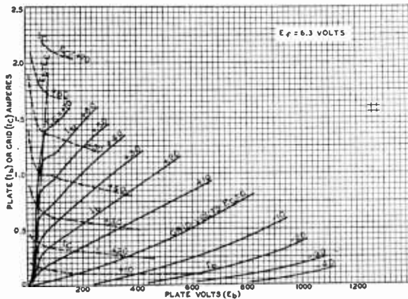
Fig. 12—Characteristic curves.
