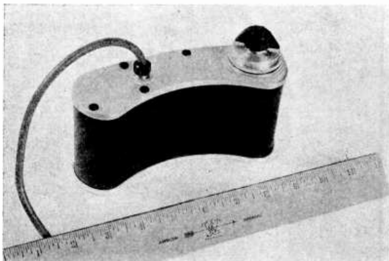
Fig. 15—5-kilovolt vibrator power supply.
