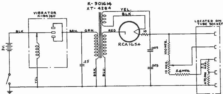
Fig. 13—Basic circuit of vibrator power supply.
