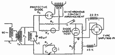
Fig. 12—Peak emission test circuit.
