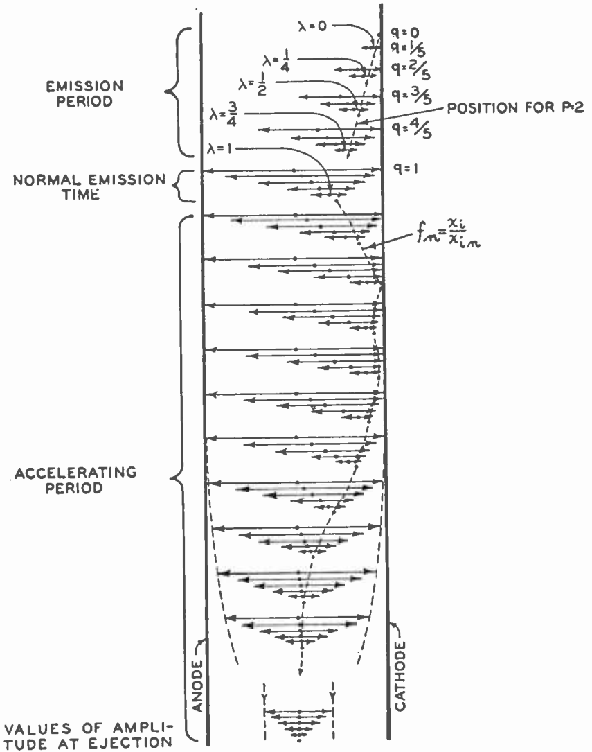
Fig. 5—Schematic history of oscillations.
