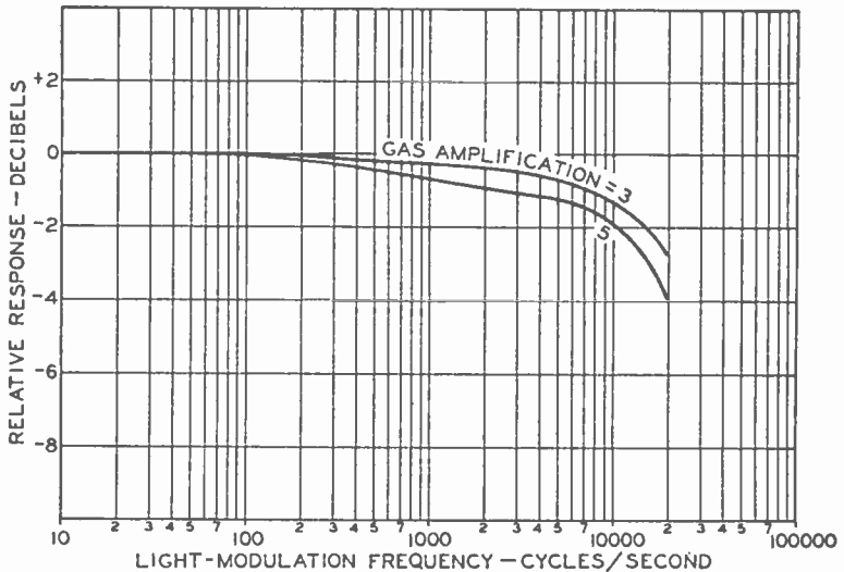
FIG. 4. Frequency response of 1P37.
