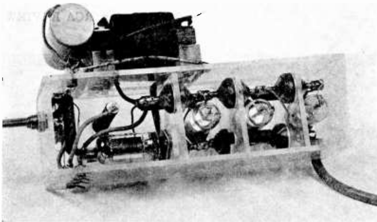
Fig. 23—16-kilovolt voltage quadrupler power supply.
