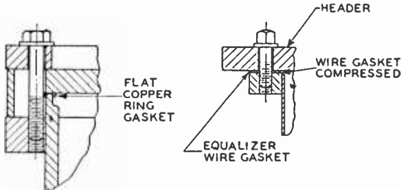
Fig. 2—Details of the copper-gasket vacuum seals.
