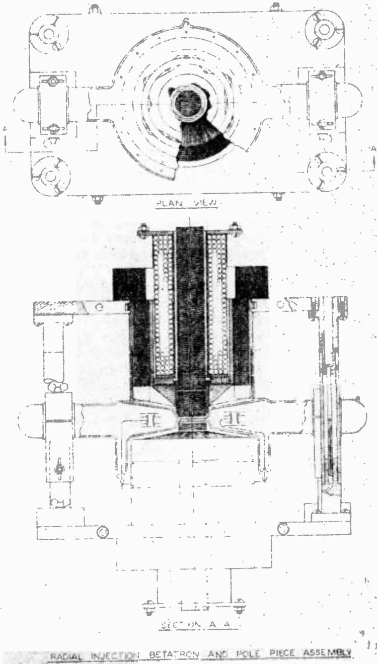
Fig. 6—Cross-section of pole pieces and tube for radial injection test.
