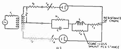
Fig. 25—Components of equivalent and practical full-wave, choke-input circuits.
