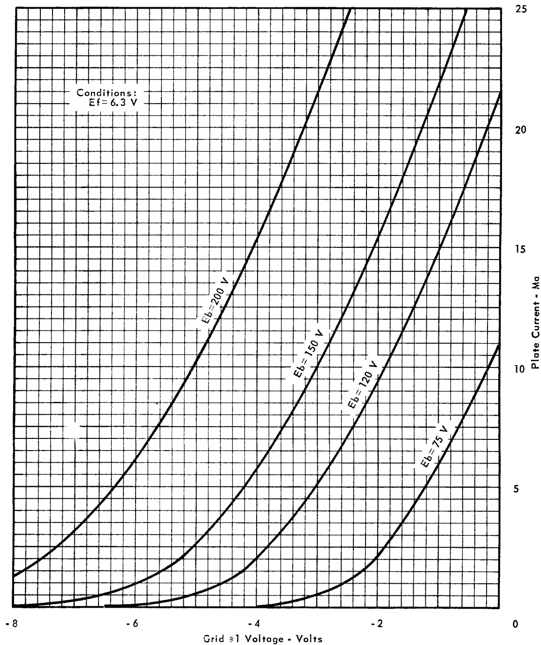
AVERAGE CHARACTERISTICS
