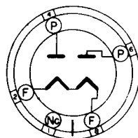
BOTTOM VIEW SHORT MEDIUM SHELL 5 PIN OCTAL
