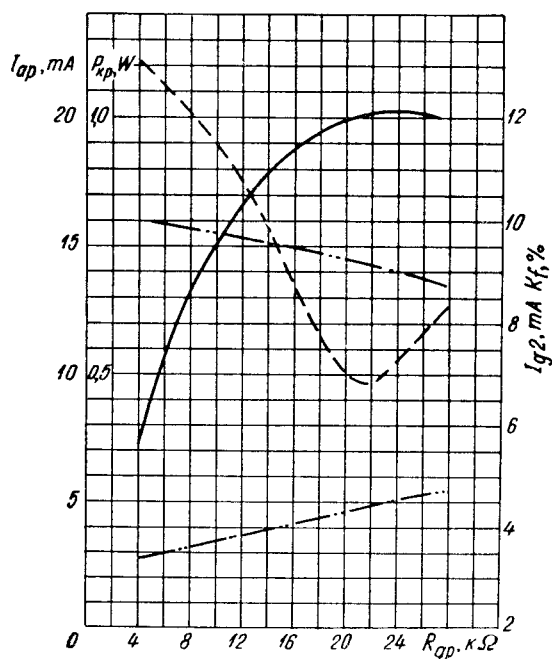
I_{ap}, I_{g2}, P_{kp}, k_{fp} = f(R_{ap}) ————— I_{ap} U_h = 6,3 \text{ V} - - - - - I_{g2} U_{ap} = 250 \text{ V} ..... P_{kp} U_{g2} = 200 \text{ V} - · - · - k_f U_{g1} = -3 \text{ V} U_{g1 \sim (eff)} = 0,9 \text{ V}
