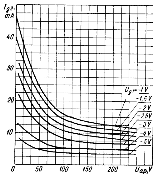
I_{g2} = f(U_{ap}) U_h = 6,3 \text{ V} U_{g2} = 240 \text{ V}
