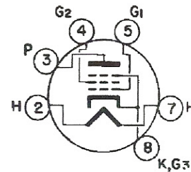
BOTTOM VIEW BASING DIAGRAM JEDEC 7AC
