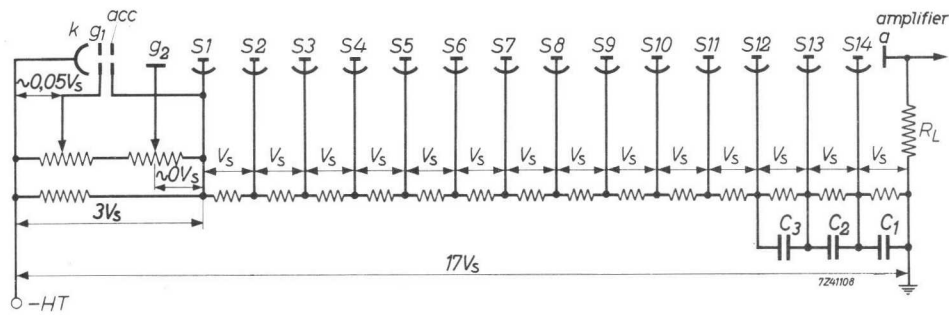
voltage divider type A 1)
