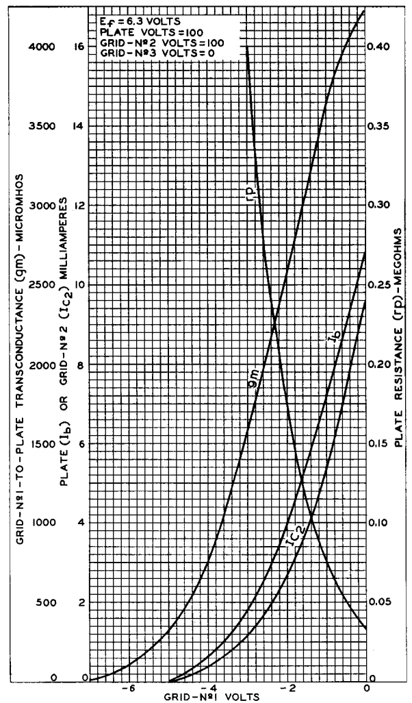
Fig.2 - Average Characteristics of Type 5636.
