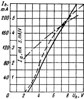
I_h, I_a, S = f(U_h) --- I_h U_a = 200 V — I_a U_g = -1 V - - - S
