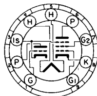
BOTTOM VIEW SMALL BUTTON 9 PIN BASE 9EG
