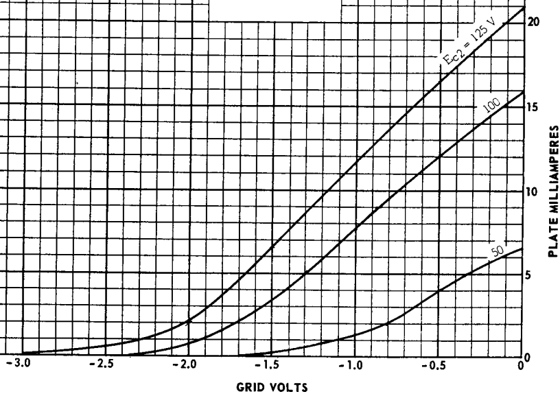
AVERAGE TRANSFER CHARACTERISTICS E_b = 125 VOLTS
