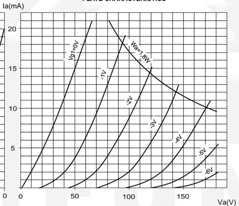
PLATE CHARACTERISTICS
