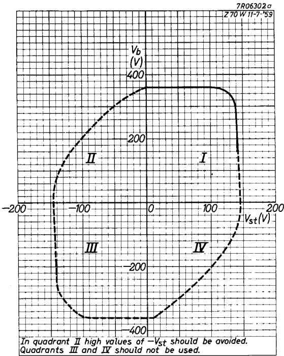
Fig. 16e. Breakdown characteristic.
