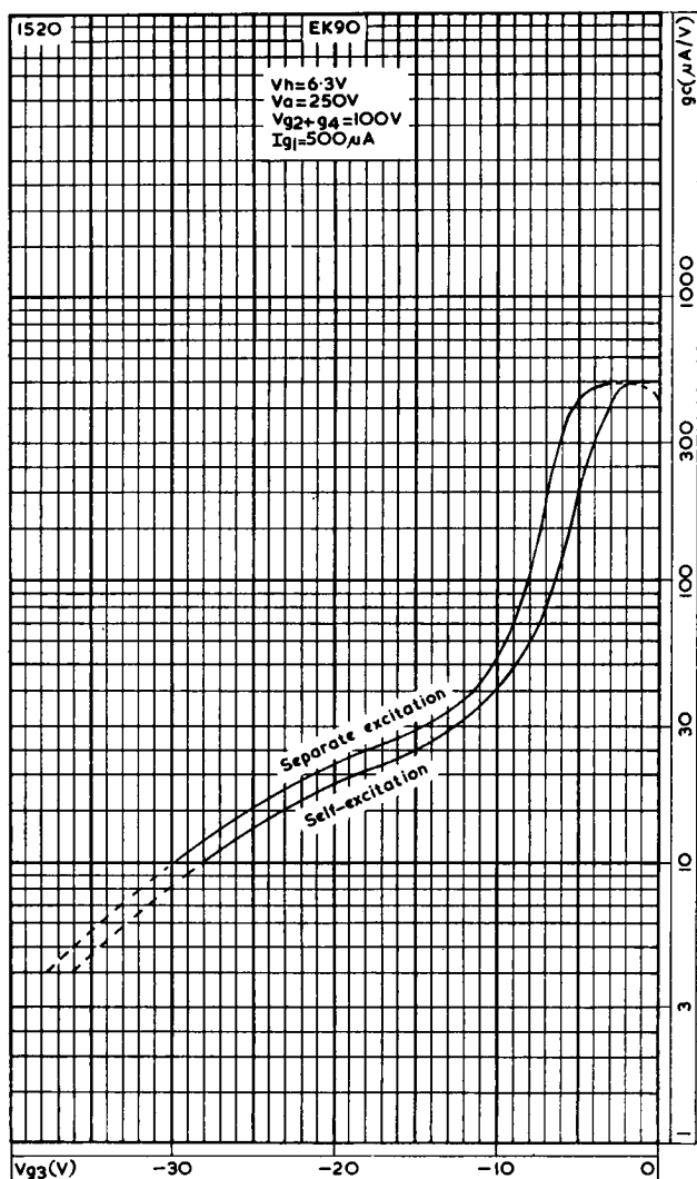
CONVERSION CONDUCTANCE PLOTTED AGAINST CONTROL GRID VOLTAGE
