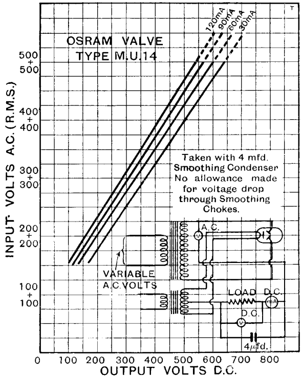
CHARACTERISTIC CURVES OF AVERAGE VALVES.
