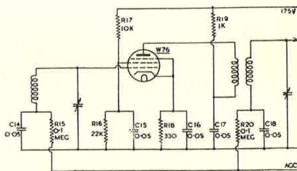
FIG. 10 RF AMPLIFIER
