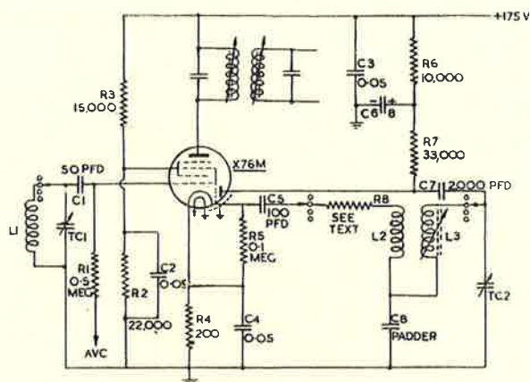
FIG. 1 NORMAL CIRCUIT
