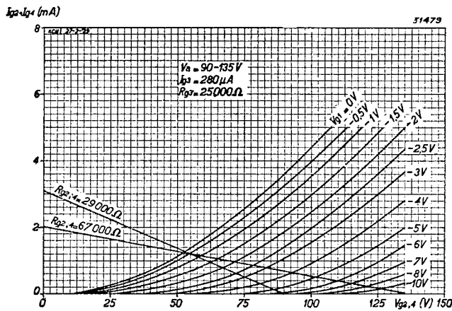
Fig. 14 Screen-grid current Ig_2 + Ig_4 as a function of the screen voltage Vg_2 , with grid bias Vg_1 as parameter. The resistance lines for Rg_{2,4} = 67,000 ohms for a battery voltage of 135 V, and for Vg_{2,4} with reference to a 90 V battery are also given.
