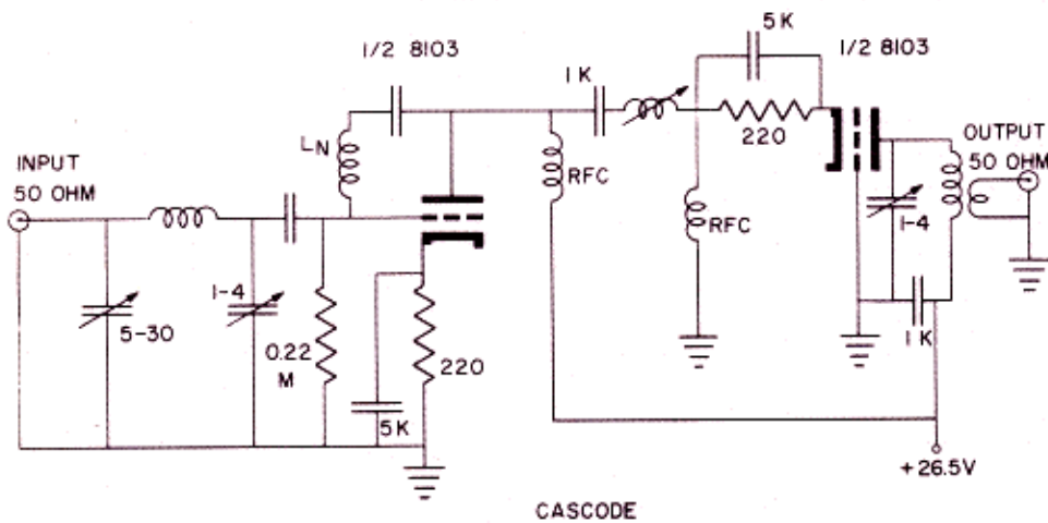
VHF CASCODE AMPLIFIER
