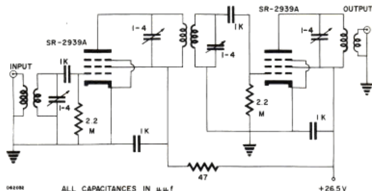
2-STAGE CASCADE IF AMPLIFIER
