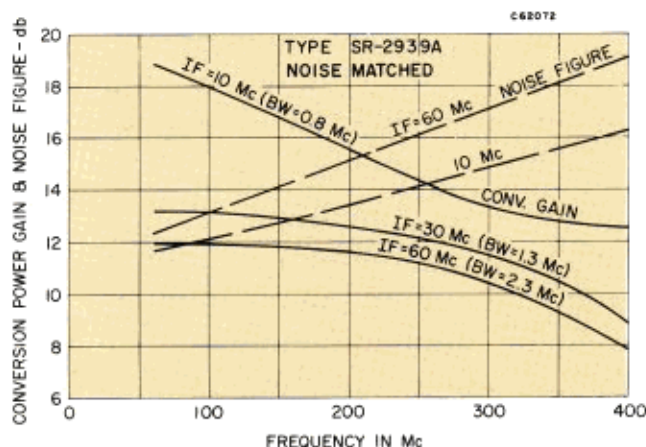
PERFORMANCE CURVE — MIXER
