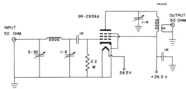
VHF AMPLIFIER — SINGLE PENTODE
