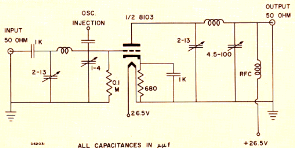
VHF TRIODE MIXER TEST CIRCUIT
