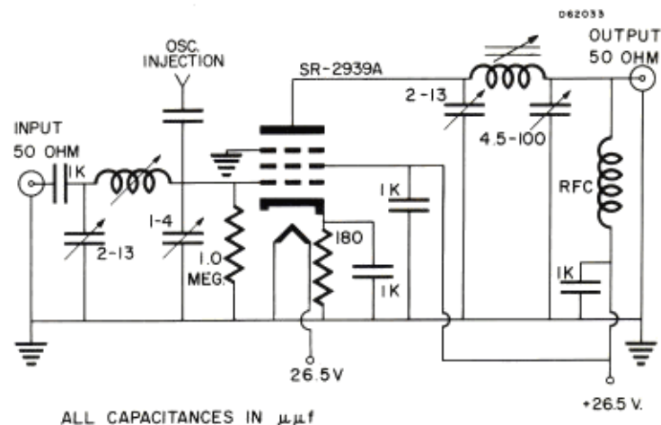
VHF PENTODE MIXER TEST CIRCUIT
